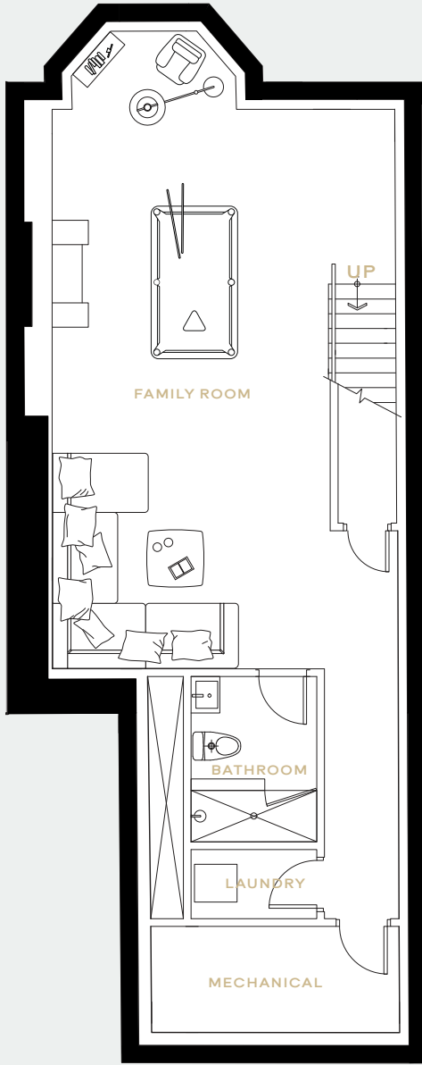
BASEMENT
